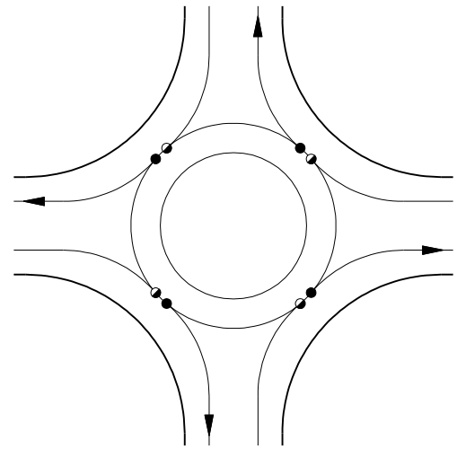
Roundabout: 8 Conflict Points
