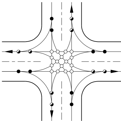
Signaled Intersection: 32 Conflict Points
